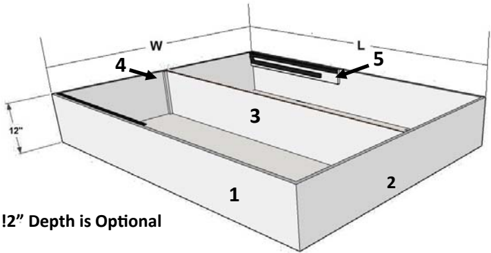
Cut List for Pedestal and Platform Parts.
